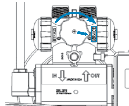
Service Position
